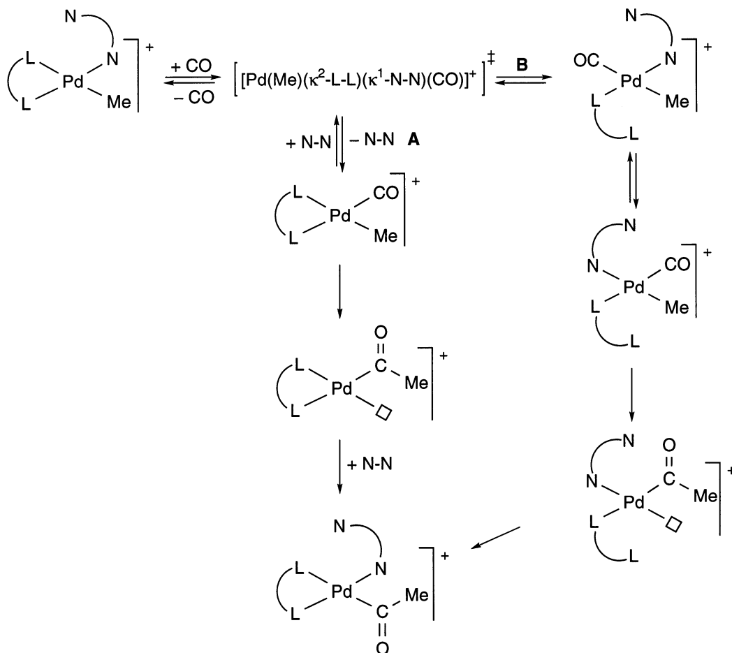
Scheme 1. Two proposed mechanisms for CO insertion reaction in complexes 1a–4a .
