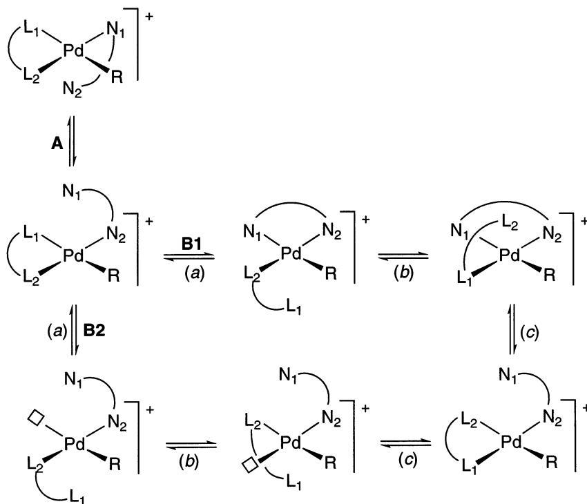
Scheme 2. Proposed mechanisms for exchange processes in complexes 1–5 .
