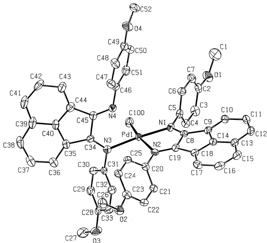
Fig. 1. ORTEP drawing (50% probability level) and adopted numbering scheme of [\text{Pd}(\text{Me})(p\text{-An-BIAN})_2]\text{SO}_3\text{CF}_3 ( 1a ); hydrogen atoms, \text{SO}_3\text{CF}_3 anion and \text{CH}_2\text{Cl}_2 have been omitted for clarity.
