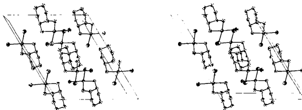
Fig. 2. The contents of the unit cell of [Pt( cis -dac)Br 2 ] 3 ·H 2 O. a * and c are parallel to the side and bottom of the page respectively and the view is down b .
