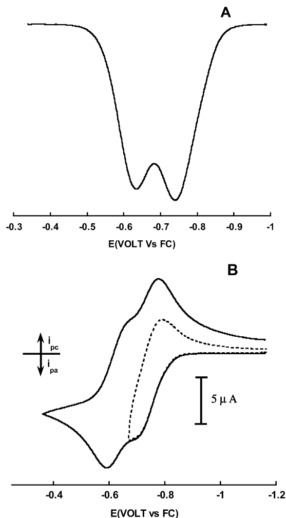
Figure 4. (A) Square-wave voltammogram of 1.6 mM 2 in \text{CH}_2\text{Cl}_2/0.05\text{M} [\text{NBu}_4][\text{B}(\text{C}_6\text{H}_3(\text{CF}_3)_2)_4] , 150 Hz, 1.5 mm GC electrode. (B) Cyclic voltammogram of 2 under the same conditions, scan rate 0.1 \text{ V s}^{-1} .
