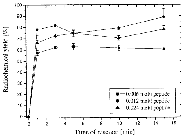
Figure 3. Time dependence of ^{18}\text{F} -fluoroethylamidation of protected [Gly-OH ^9 ]oxytocin in presence of TBTU, n = 3-4 , conditions: 250 \mu\text{l} DMF, 20°C, [Gly-OH ^9 ]oxytocin/TBTU/TEA = 1/1/2
