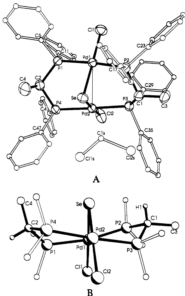
Figure 2. (a) Structure of anti -Pd 2 Cl 2 (μ-Se)(dpmMe) 2 ( 2d ). Only the ipso C atoms of the phenyl rings are labeled, and H atoms are omitted for clarity. Thermal ellipsoids are drawn at the 50% probability level. (b) Side view showing conformations of the rings and CH(Me) moieties.
