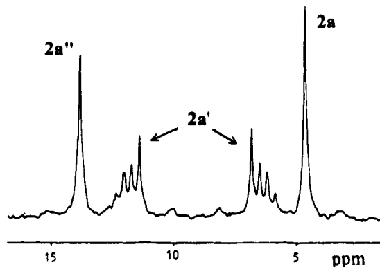
Figure 1. ^{31}\text{P}\{^1\text{H}\} NMR spectrum of the product mixture from 2.5 h reaction of \text{Pd}_2\text{Cl}_2(\text{dpm})_2 ( 1a ) with a 15-fold excess of \text{H}_2\text{Se} at ambient conditions.
