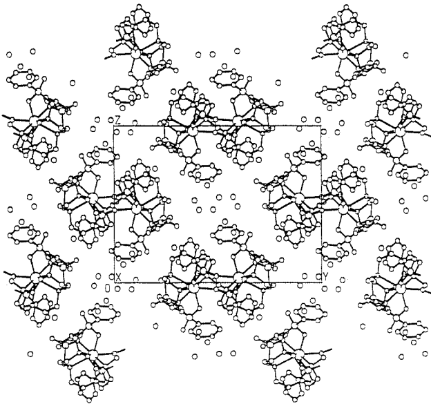
Fig. 3 Crystal packing of [YbL] 2 ·6H 2 O (view along the y axis).
