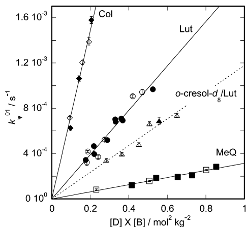
Figure 3. Pseudo-first-order rate constants, k_{\psi}^{01} , for H/D exchange of MTO as a function of [B] and [D] in benzene- d_6 . The solid lines show k_{\psi}^{01} with D = C_6D_5OD and the indicated base catalysts. The dashed line refers to the system o -cresol- d_8 /Lut. Solid symbols, [D] = 1.0 mol kg^{-1} ; open symbols, [D] = 0.5–1.4 mol kg^{-1} .
