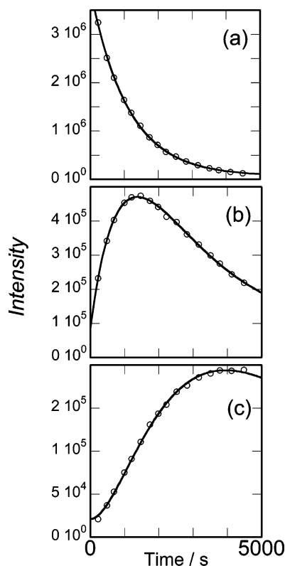
Figure 2. ^1\text{H} NMR signal intensities (arbitrary units) vs time for (a) MTO, (b) MTO- d , and (c) MTO- d_2 in benzene- d_6 at 298.0 K. Concentrations: 0.0175 mol \text{kg}^{-1} of MTO, 1.35 mol \text{kg}^{-1} of \text{C}_6\text{D}_5\text{OD} , 0.312 mol \text{kg}^{-1} of Lut. Curve fittings from eqs 1–3 correspond to (a) k_{\psi}^{01} = 9.05 \times 10^{-4} \text{ s}^{-1} , (b) k_{\psi}^{12} = 5.77 \times 10^{-4} \text{ s}^{-1} , and (c) k_{\psi}^{23} = 2.47 \times 10^{-4} \text{ s}^{-1} , with each rate constant relying on its predecessor(s), as explained in the text.
