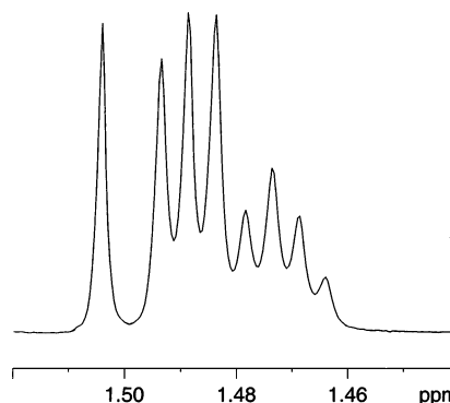
Figure 1. ^1\text{H} NMR spectra of \text{MTO-}d_n ( n = 0\text{--}2 ) after 7 h at 323 K. Concentrations: 0.05 mol \text{kg}^{-1} of MTO, 1.0 mol \text{kg}^{-1} of \text{CD}_3\text{OD} , 0.6 mol \text{kg}^{-1} of pyridine- d_5 .
