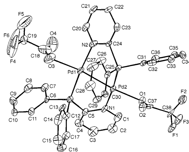
Fig. 2 Molecular structure and atom labelling scheme of [Pd 2 (Ph 2 PC 5 H 4 N) 2 (O 2 CCF 3 ) 2 ]. Hydrogen atoms are omitted for clarity.
