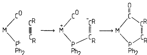
Scheme 1. Proposed mechanism for the reaction of the phosphido complexes with alkynes.
