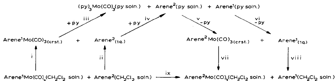
Scheme 1. Thermochemical cycle for calculation of enthalpies of arene exchange in methylene chloride. i: -\Delta H(\text{C}^1)(\text{soln. CH}_2\text{Cl}_2) ; ii: -\Delta H(\text{A}^2)(\text{soln. CH}_2\text{Cl}_2) ; iii: \Delta H(\text{C}^1)(\text{react. py}) ; iv: \Delta H(\text{A}^2)(\text{soln. py}) ; v: -\Delta H(\text{C}^2)(\text{react. py}) ; vi: -\Delta H(\text{A}^1)(\text{soln. py}) ; vii: \Delta H(\text{C}^2)(\text{soln. CH}_2\text{Cl}_2) ; viii: \Delta H(\text{A}^1)(\text{soln. CH}_2\text{Cl}_2) ; ix: \Delta H(\text{C}^1 + \text{A}^2 \rightarrow \text{C}^2 + \text{A}^1)(\text{exchange}) .
