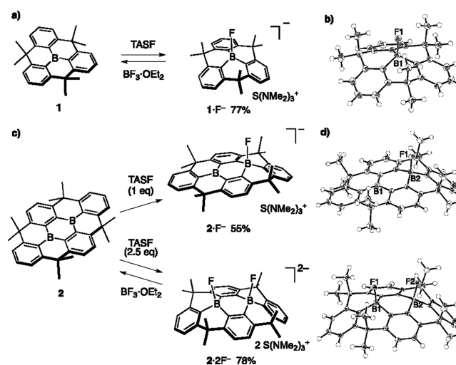
Figure 3. Plane-to-bowl conversion by fluoride ion coordination in 1 and 2 . (a) Reaction of 1 with a fluoride ion to form 1\cdot\text{F}^-/\text{S}(\text{NMe}_2)_3^+ . (b) Crystal structure of 1\cdot\text{F}^-/\text{S}(\text{NMe}_2)_3^+ . (c) Reactions of diborane 2 with 1 equiv or an excess of fluoride ion to produce 2\cdot\text{F}^-/\text{S}(\text{NMe}_2)_3^+ or 2\cdot 2\text{F}^-/2\text{S}(\text{NMe}_2)_3^+ , respectively. (d) Crystal structures of 2\cdot\text{F}^-/\text{S}(\text{NMe}_2)_3^+ and 2\cdot 2\text{F}^-/2\text{S}(\text{NMe}_2)_3^+ . In the ORTEP drawings in (b) and (d), the thermal ellipsoids are drawn at the 50% probability level, and the counteranions are omitted for clarity.
