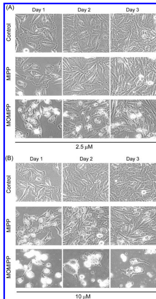
Figure 3. Comparison of the abilities of MOMIPP and MIPP to induce the morphological hallmarks of methuosis. One day after plating, U251 GBM cells were treated with MOMIPP or MIPP at final concentrations of 2.5 (A) or 10 \mu M (B). Controls received an equivalent volume of vehicle (DMSO). Cells were observed by phase contrast microscopy on three sequential days after addition of the compounds, without changing the medium or replenishing the compounds. Methuosis is characterized by extensive accumulation of phase-lucent cytoplasmic vacuoles, with eventual cell rounding and detachment from the substratum as viability is compromised. 6,10
