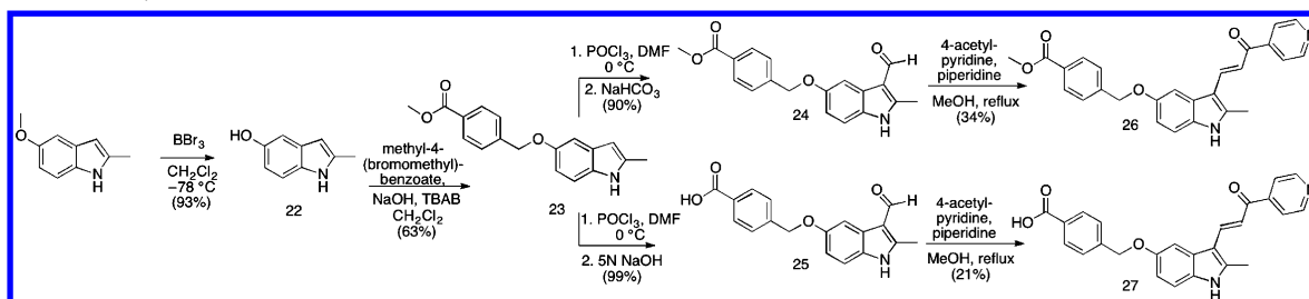
Scheme 2. Analogues with 5' Modifications of the Indole Ring Generated by Functionalizing the Indole Prior to Introduction of the Pyridine Moiety a
