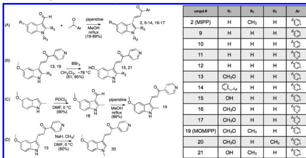
Scheme 1. Synthesis of Analogues of MIPP (Compound 2 ) a
