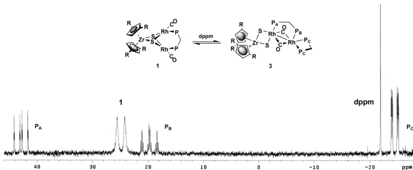
Figure 2. ^{31}\text{P}\{^1\text{H}\} NMR spectrum of the equilibrium 1 + \text{dppm} \rightleftharpoons 3 observed in the reaction of [\text{Cp}^*\text{Zr}(\mu_3\text{-S})_2\{\text{Rh}(\text{CO})_2\}_2] with 2 mol equiv of dppm in \text{C}_6\text{D}_6 .
