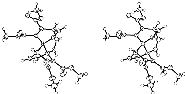
Fig. 1. Stereoscopic projection of the X-ray structure of tetramethyl (1RS,2RS,5SR,8RS)-tetracyclo[6.2.2.2 2,5 .0 1,5 ]tetradeca-3,6,9,11,13-pentaene-3,4,9,10-tetracarboxylate ('anti'-7)
