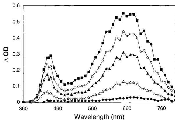
Figure 1. Transient absorption spectra from the LFP (355 nm, 1–5 mJ, 6 ns) of 2 in CH 3 CN taken 100 ns (■), 800 ns (◇), 1.6 \mu s (▲), 3.2 \mu s (△), and 6.4 \mu s (●) following the excitation pulse.
