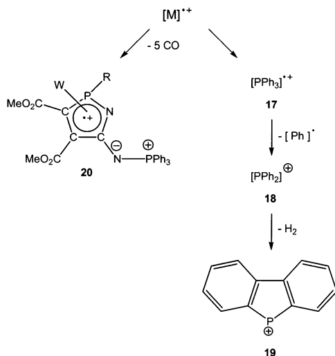
Scheme 8. Fragmentation of the Molecular Radical Cations of 11a–d
