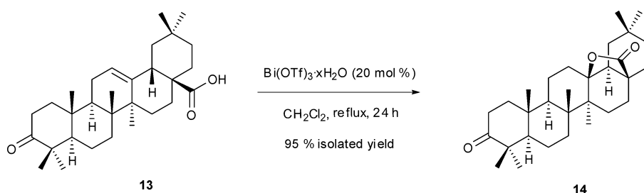
Scheme 3 \text{Bi}(\text{OTf})_3 \cdot x\text{H}_2\text{O} -promoted lactonization of oleanonic acid 13 .
