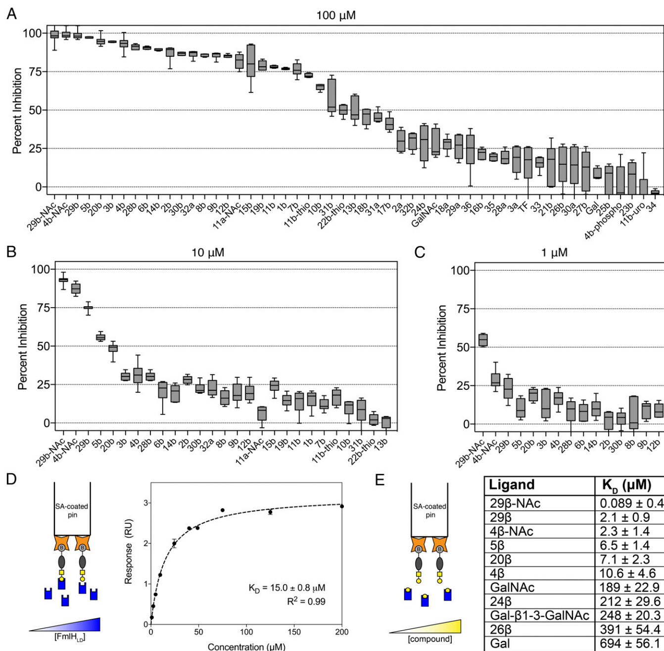
Fig. 3. In vitro screening and affinity determination of galactosides against FmlH LD . (A–C) ELISA-based competition assay performed in triplicate in the absence or presence of (A) 100 μM, (B) 10 μM, and (C) 1 μM compounds with at least two biological replicates. Data are reported as the mean percent inhibition, with the box indicating the 25th to 75th percentiles and the whiskers indicating the 2.5th and 97.5th percentiles. a, α; b, β. (D, Left) Schematic of conventional BLI experiment, in which pins coated with streptavidin (orange stars) are loaded with biotinylated Ser-TF (gray ovals and yellow square-circle conjugates) and dipped into solutions of varying concentrations of FmlH LD (blue rectangles). (Right) Equilibrium analysis of soluble FmlH LD binding to immobilized Ser-TF according to a 1:1 binding model. (E, Left) Schematic of competitive BLI experiment, in which streptavidin-coated pins are dipped into a solution composed of a fixed concentration of FmlH LD in the presence of varying concentrations of galactoside (yellow circles). (Right) Equilibrium constants of soluble galactoside-mediated inhibition of FmlH LD in binding immobilized Ser-TF in accord with R^2 > 0.85 .
