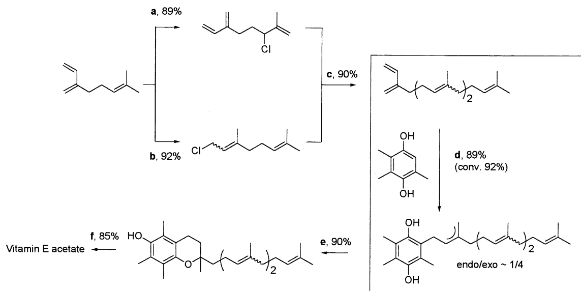
Scheme 2. A convergent vitamin E synthesis. a a Reagents and conditions: (a) \text{Cl}_2 (g), pentane, reflux; (b) \text{CuCl} (5 mol%), \text{HCl} (g), \text{CH}_2\text{Cl}_2 , 0^\circ\text{C} ; (c) \text{Mg}^\circ , THF, -20^\circ\text{C} then \text{CuCl} (5 mol%); (d) [\text{RhCl}(\text{COD})]_2 (0.5 mol%), \text{dppb} (0.7 mol%), \text{K}_2\text{CO}_3 (20 mol%), toluene, 110^\circ\text{C} ; (e) \text{MeAlCl}_2 or p\text{TSA} (5 mol%), hexane, 100^\circ\text{C} ; (f) \text{H}_2 (20 atm.), \text{Pd/C} (2 mol%), \text{EtOH} then \text{Ac}_2\text{O} (1.2 equiv.), \text{Et}_3\text{N} (1.5 equiv.), 25^\circ\text{C}
