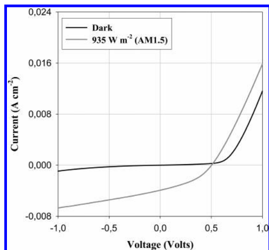
FIGURE 3. IV curves of the device based on 35 and PCBM (1:4) in the dark and under illumination with a sun simulator at 935 W m -2 approximating AM1.5 conditions.
