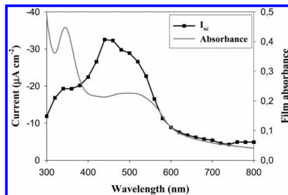
FIGURE 4. Photovoltaic action spectrum in terms of the short circuit current ( I_{sc} ) for a photovoltaic cell based on a mixture of 35 and PCBM (1:4) with an active area of 3 cm 2 . The UV-vis spectrum of the device film is also shown.
