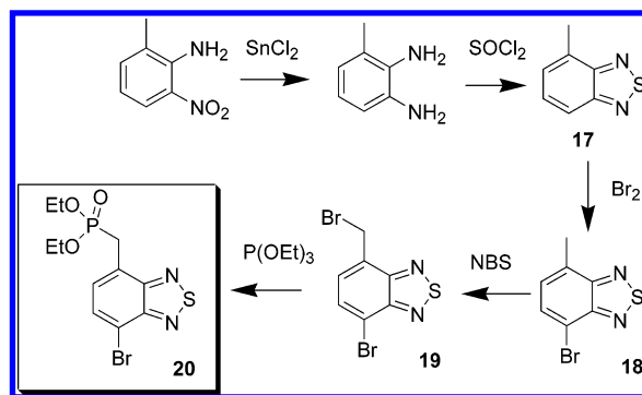
SCHEME 5. Synthesis of the Dipropyl- and Dipropoxyphenylvinylstannane Reagents
