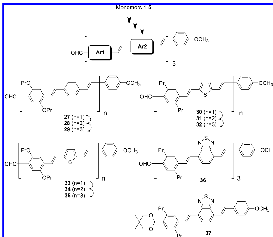
CHART 2. Structures of the Four Different Types of “Homo” Oligomers Prepared in This Study Based on the Monomers 2–5 a
