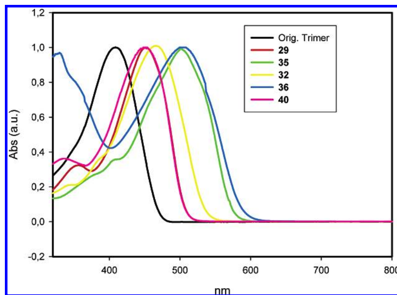
FIGURE 2. Normalized absorption spectra of the original trimer prepared from monomer 1 and the trimers 29 , 32 , 35 , 36 , and 40 dissolved in chloroform.
