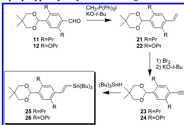
SCHEME 5. Synthesis of the Dipropyl- and Dipropoxyphenylvinylstannane Reagents
