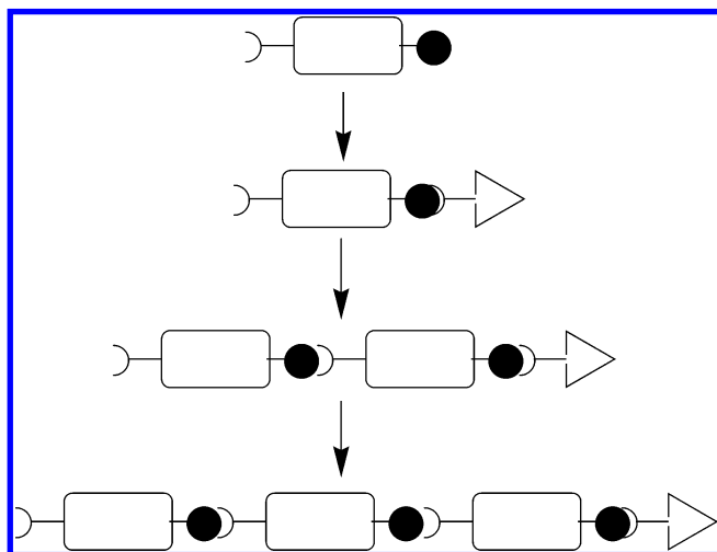
FIGURE 1. Concept of unidirectional stepwise oligomerization. A monomer has two different end groups that can be coupled in a sequential manner. One group is protected during coupling and then deprotected to allow the next cycle. In the first reaction, the monomer is end-capped with a monofunctional reagent.
