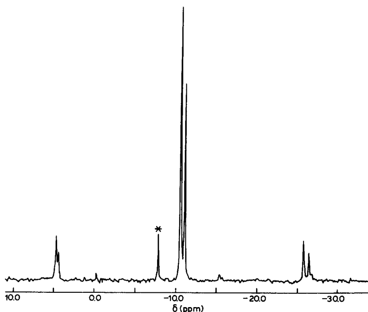
Fig. 2. 31 P{ 1 H} NMR of Mc 2 Pt 2 (μ-Cl) 2 (PMc 2 Ph) 2 .
