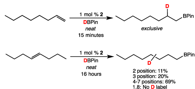
Scheme 2. Catalytic Hydroboration of 1- and 4-Octene with DBPin in the Presence of 2
