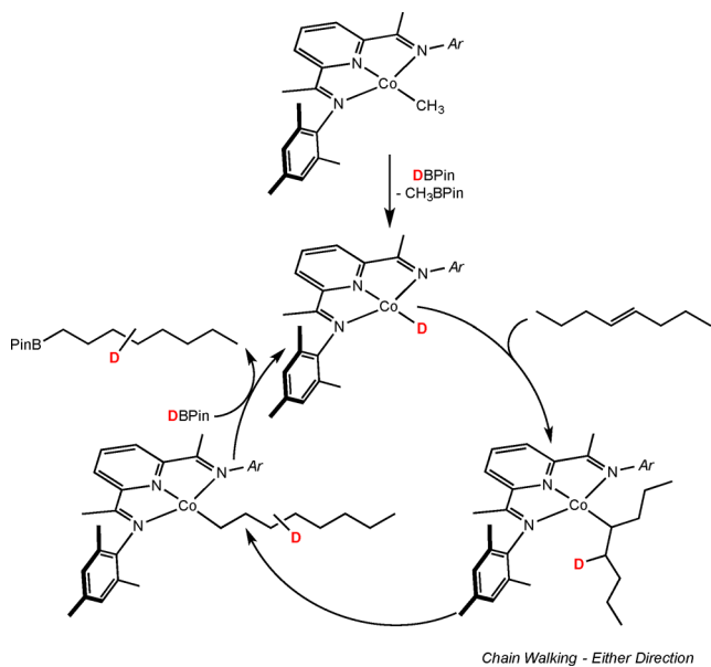
Scheme 3. Proposed Mechanism for Bis(imino)pyridine Cobalt-Catalyzed Alkene Hydroboration with DBPin Accounting for the Observed Preference for Terminal Selectivity
