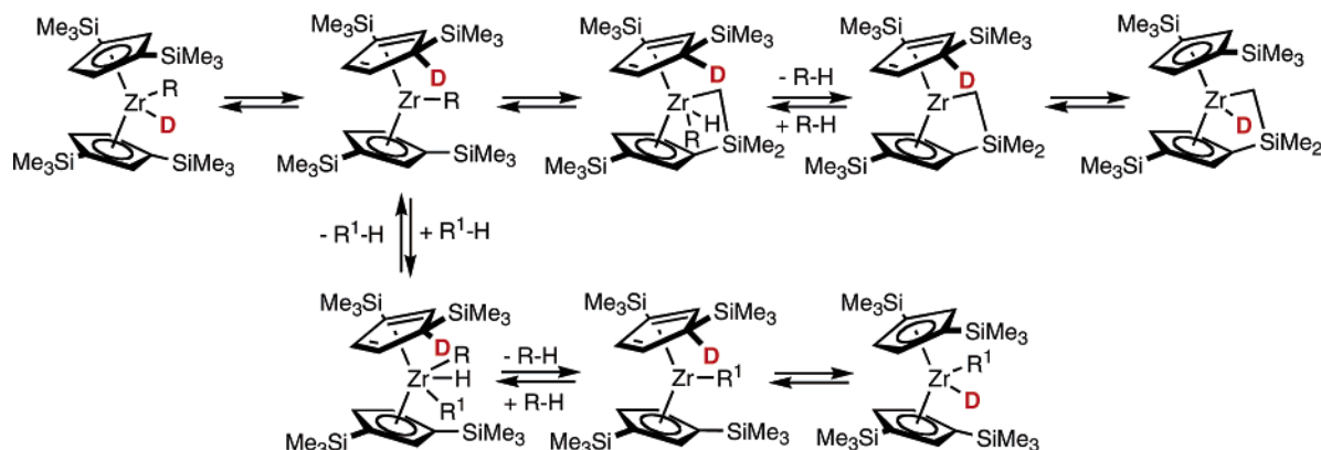
Figure 5. Cyclometalated-assisted pathway for alkane reductive elimination from zirconocene alkyl hydride complexes.
