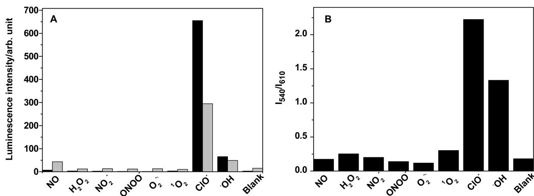
Figure 6. (A) Luminescence intensities of the products of AMTTA-Tb 3+ (10 \mu M, black column) and AMTTA-Eu 3+ (10 \mu M, gray column) reacted with various ROS in 50 mM HEPES buffer of pH 7.2. (B) I_{540}/I_{610} ratios of the products of the AMTTA-Eu 3+ /Tb 3+ mixture (total concentration of 20 \mu M, Tb 3+ /Eu 3+ = 1/1) reacted with various ROS in 50 mM HEPES buffer of pH 7.2.
