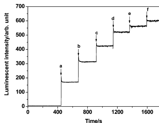
Figure 4. Time course of the luminescence response of AMTTA-Tb 3+ ( 10 \mu\text{M} ) to the addition of ClO − in 50 mM HEPES buffer of pH 7.2 at room temperature (the 3.0 \mu\text{M} ClO − solution was added six times at a, b, c, d, e, and f, respectively). The luminescence intensity at 540 nm was determined ( \lambda_{\text{ex}} = 331 \text{ nm} ).
