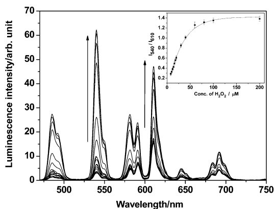
Figure 2. Time-gated emission spectra ( \lambda_{\text{ex}} = 331 \text{ nm} ) of the AMTTA-Eu 3+ /Tb 3+ mixture (total concentration of 20 \mu\text{M} , Tb 3+ /Eu 3+ = 1/1) in the presence of Fe 2+ ( 60 \mu\text{M} ) and different concentrations of H 2 O 2 (0.0, 2.0, 4.0, 6.0, 8.0, 10, 12, 14, 16, 18, 20, 30, 40, 60, 80, 100, and 200 \mu\text{M} ) in 50 mM HEPES buffer of pH 7.2. The inset shows the intensity ratio of I_{540}/I_{610} as a function of the H 2 O 2 concentration.
