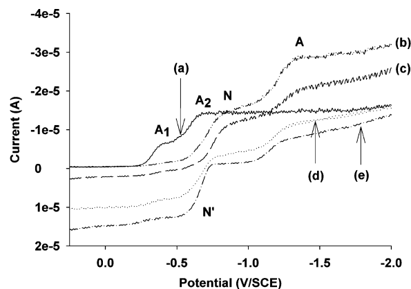
Figure 4. (a) RDE voltammograms of [\text{Pd}_3]^{2+} (scan rate = 0.02 \text{ V s}^{-1} ) in THF/ \text{Bu}_4\text{NPF}_6 solution at room temperature and after (b) the addition of 1 equiv of \text{Pd}_2\text{Cl}_2 , (c) 1-electron reduction at -0.8 \text{ V} , (d) 2-electron reduction at -0.8 \text{ V} , and (e) 2.6-electron reduction at -0.8 \text{ V} . Starting potential: 0.2 \text{ V}
