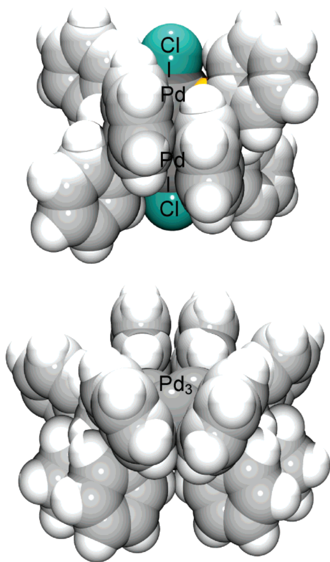
Figure 3. Space filling models for 1^{2+} and 2 showing the screening of the Cl ligand on 2 preventing good interactions with the \text{Pd}_3 center. This conformation is the one that shows the largest possible cavity size. This global conformation depends on the dppm conformation.
