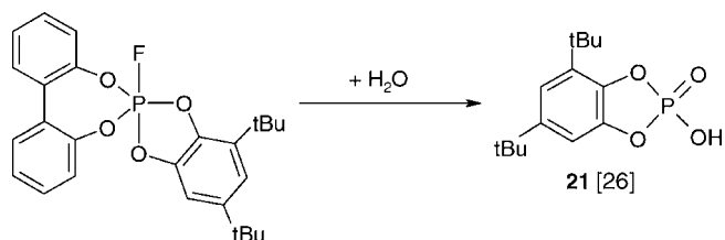
SCHEME 8 Hydrolysis of a fluoro phosphorane.
