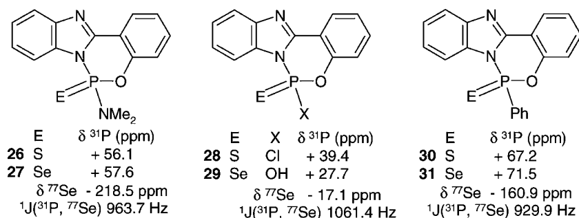
SCHEME 11 ^{31}\text{P} and ^{77}\text{Se} NMR data for compounds 26–31 .
