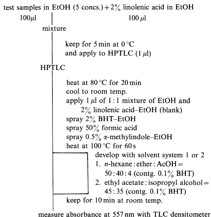
Fig. 3. Testing Procedure for the Determination of Antioxidative Activity using \alpha -Methylindole Reagent and HPTLC
