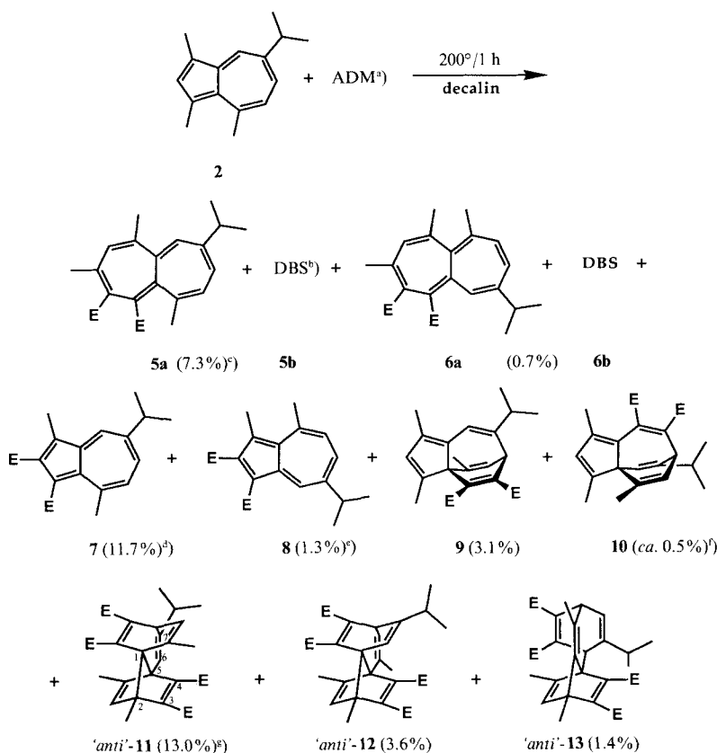
Scheme 3 a)
