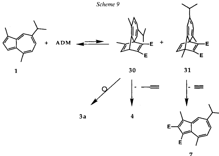
Scheme 9
