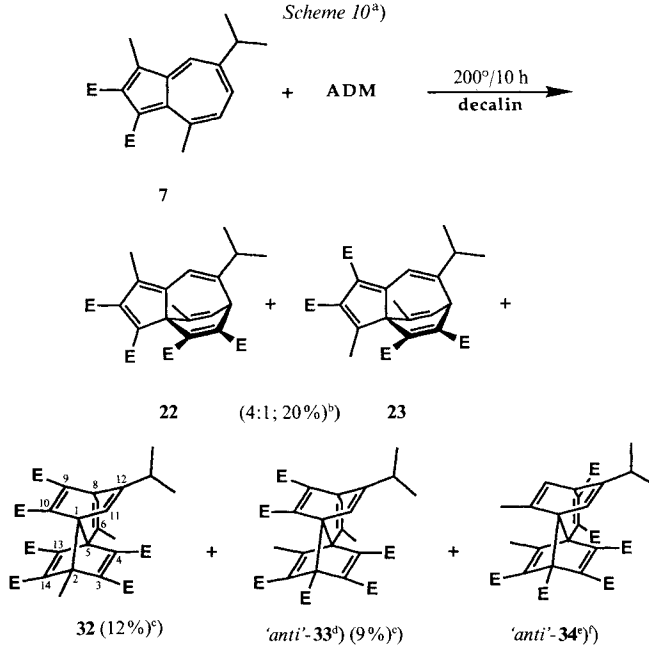
Scheme 10 a)
