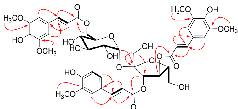
Figure 2. Key 1 H- 1 H COSY (bold) and HMBCs (→) of 1 .
