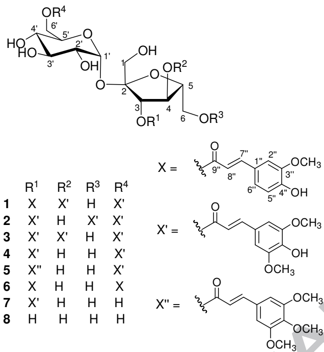
Figure 1. Chemical structures of 1-8 .
