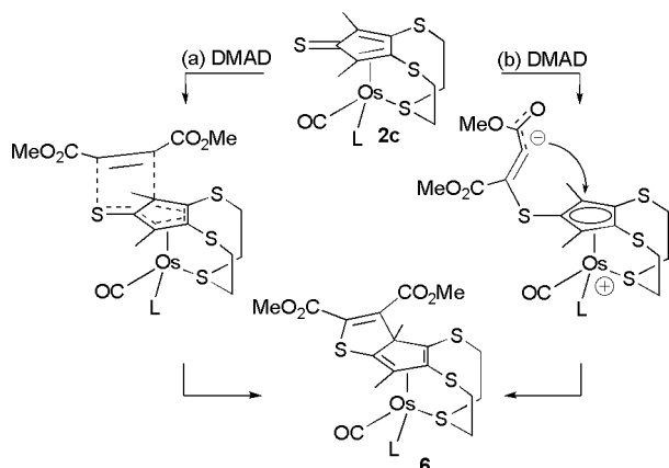
Scheme 2. (a) Concerted vs (b) Zwitterionic Routes for the Cycloaddition of DMAD to 2c
