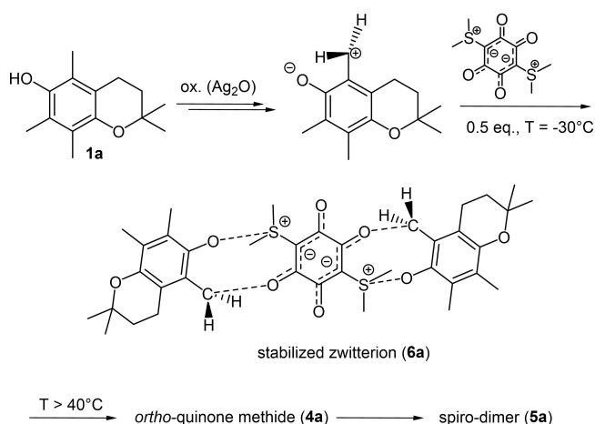
Scheme 4. Zwitterionic intermediate 6a stabilized by electrostatic interaction with another zwitterion, before bond rotation leads on to oQM 4a and further dimerization to spiro-dimer 5a .
