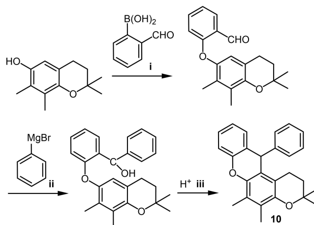
Scheme 8. Three-step synthesis of xanthene 10 for independent structure confirmation. i = \text{Cu}(\text{OAc})_2 , \text{NEt}_3 , DCM, r.t., 17 h, ii = THF, r.t. 30 min, iii = cat. \text{H}_2\text{SO}_4 conc., 0^\circ\text{C} , 5 min.
