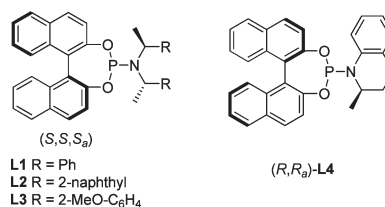
Fig. 2 Chiral phosphoramidite ligands.
