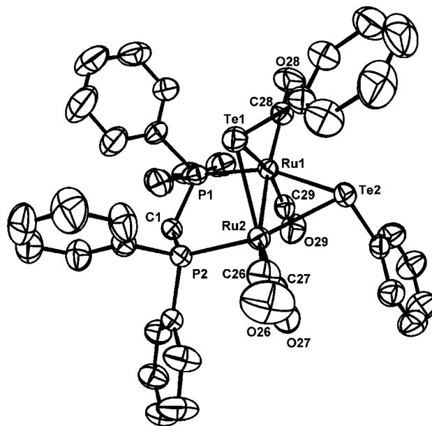
Figure 1. ORTEP diagram of [\text{Ru}_2(\text{CO})_4(\mu\text{-TePh})_2(\mu\text{-dppm})] ( 2 ) with 50% probability thermal ellipsoids. Selected interatomic distances ( \text{\AA} ) and angles (deg): \text{Ru}(2)\text{--Ru}(1) = 2.7475(9) , \text{Ru}(2)\text{--Te}(2) = 2.6745(11) , \text{Ru}(1)\text{--Te}(2) = 2.6753(10) , \text{Ru}(1)\text{--Te}(1) = 2.6691(8) , \text{Ru}(2)\text{--Te}(1) = 2.6988(8) , \text{Ru}(2)\text{--C}(27) = 1.880(7) , \text{Ru}(2)\text{--C}(26) = 1.888(7) , \text{Ru}(2)\text{--P}(2) = 2.3172(17) , \text{Ru}(1)\text{--C}(29) = 1.872(6) , \text{Ru}(1)\text{--C}(28) = 1.894(6) , \text{Ru}(1)\text{--P}(1) = 2.3162(18) ; \text{Ru}(2)\text{--Te}(2)\text{--Ru}(1) = 61.80(3) , \text{Ru}(1)\text{--Te}(1)\text{--Ru}(2) = 61.57(2) , \text{P}(2)\text{--Ru}(2)\text{--Te}(2) = 153.47(4) , \text{P}(2)\text{--Ru}(2)\text{--Te}(1) = 92.31(4) , \text{Te}(2)\text{--Ru}(2)\text{--Te}(1) = 79.88(2) , \text{P}(2)\text{--Ru}(2)\text{--Ru}(1) = 95.12(4) , \text{Te}(2)\text{--Ru}(2)\text{--Ru}(1) = 59.113(19) , \text{Te}(1)\text{--Ru}(2)\text{--Ru}(1) = 58.68(2) , \text{Te}(1)\text{--Ru}(1)\text{--Te}(2) = 80.40(2) , \text{P}(1)\text{--Ru}(1)\text{--Ru}(2) = 94.17(4) , \text{Te}(1)\text{--Ru}(1)\text{--Ru}(2) = 59.747(16) , \text{Te}(2)\text{--Ru}(1)\text{--Ru}(2) = 59.08(2) , \text{P}(2)\text{--C}(1)\text{--P}(1) = 114.9(3) .
