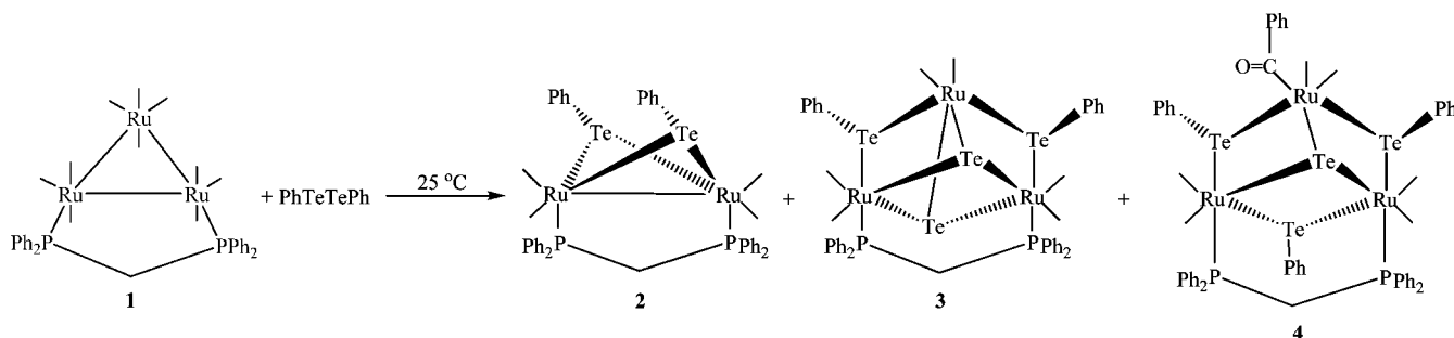
Scheme 1
