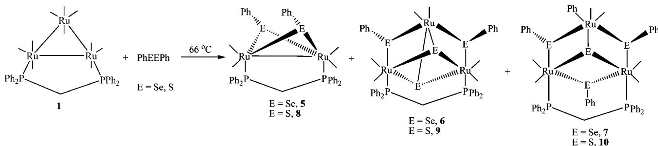
Scheme 2
