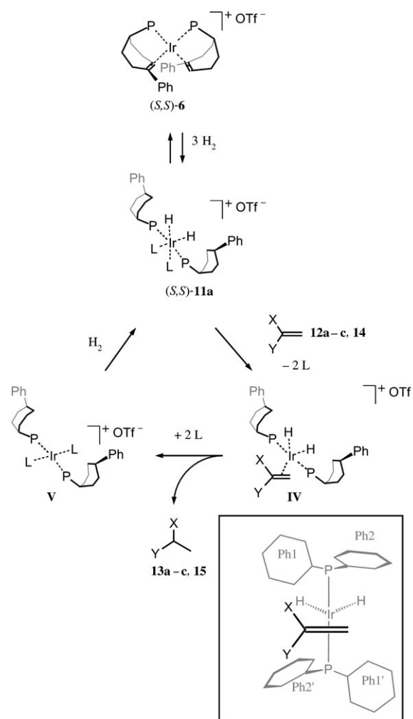
Scheme 6. Proposed mechanism for the catalytic hydrogenation of alkenes with (S,S)\text{-6} as catalyst precursor. L stands for loosely bound unspecified ligands (solvent molecules).
