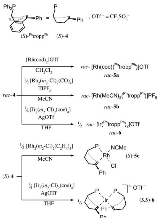
Scheme 3. Synthesis of chiral (\text{Ph-tropp}^{\text{Ph}}) \text{Rh}^{\text{I}} ( 5a–c ) and \text{Ir}^{\text{I}} complexes ( 6 ). coe = cyclooctene.
