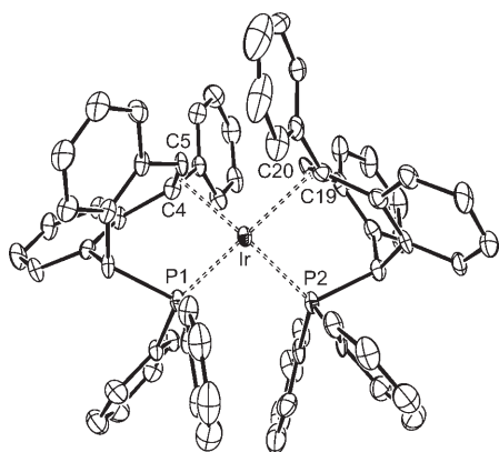
Figure 2. ORTEP plot of (S,S)\text{-[Ir(Ph-tropp)}_2\text{]OTf} ( (S,S)\text{-6} ). The thermal ellipsoids are shown at the 30% probability level. The R,R isomer, the hydrogen atoms, the triflate anion, and two molecules of dichloromethane have been omitted for clarity. Selected bond lengths [Å] and angles [°]: Ir–P1 2.263(3), Ir–P2 2.271(3), Ir–C4 2.40(1), Ir–C5 2.29(1), Ir–C19 2.47(1), Ir–C20 2.34(1), Ir–ct1 2.24(1), Ir–ct2 2.30(1) (ct1 = centroid of C4=C5, ct2 = centroid of C19=C20); P1–Ir–ct1 88.6(1), ct1–Ir–ct2 95.1(1), ct2–Ir–P2 88.6(1).
