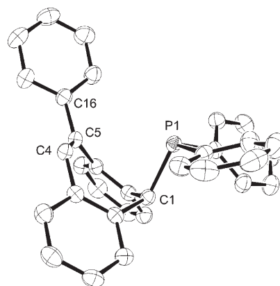
Figure 1. ORTEP view of the S enantiomer of 4 . The thermal ellipsoids are drawn at the 50% probability level. The hydrogen atoms have been omitted for clarity. Selected bond lengths [Å]: P1–C1 1.894(2), C4–C5 1.344(2), C4–C16 1.491(2). The bite angle of 4 is 75.5°.
