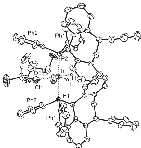
Figure 3. ORTEP plot of (S,S)\text{-}[\text{Ir}(\text{H})_2(\text{OTf})(\text{CH}_2\text{Cl}_2)(\text{H}_2\text{-tropph})_2] ( 11c ); thermal ellipsoids are shown at the 30% probability level. The R,R isomer, the hydrogen atoms of the \text{H}_2\text{-tropph} ligands, and a molecule of \text{CH}_2\text{Cl}_2 have been omitted for clarity. The hydrogen atoms bonded to the iridium are shown in calculated positions. Selected bond lengths [Å] and angles [°]: Ir1–P1 2.315(2), Ir–P2 2.313(2), Ir–Cl1 2.550(3), Ir–O1 2.260(6); O1–Ir–P2 92.1(2), O1–Ir–P1 94.7(2), P2–Ir–P1 172.7(1), O1–Ir–Cl1 88.2(2), P2–Ir–Cl1 93.5(1), P1–Ir–Cl1 89.2(1).
