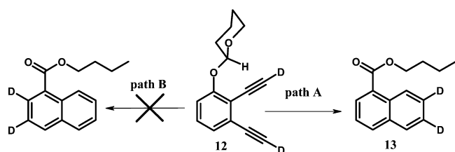
Scheme 6. Bergman Cyclization of Enediyne 2-d 2 ( 12 )
