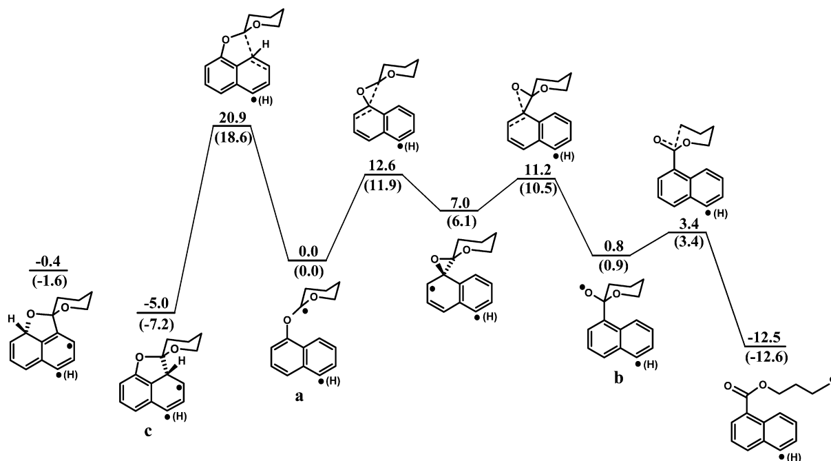
Scheme 5. Summary of Computational Study at the UB3LYP/6-31G** Level of Theory that Favors Pathway A (O-Neophyl Rearrangement) Over B a
