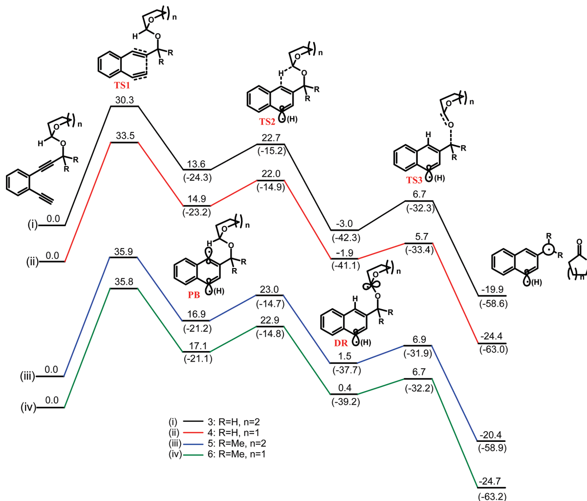
Scheme 13. Summary of the Computational Results for the Cycloaromatization/H-Abstraction Reaction for Enediynes 3–6 at the UB3LYP/6-31G** Level of Theory a
