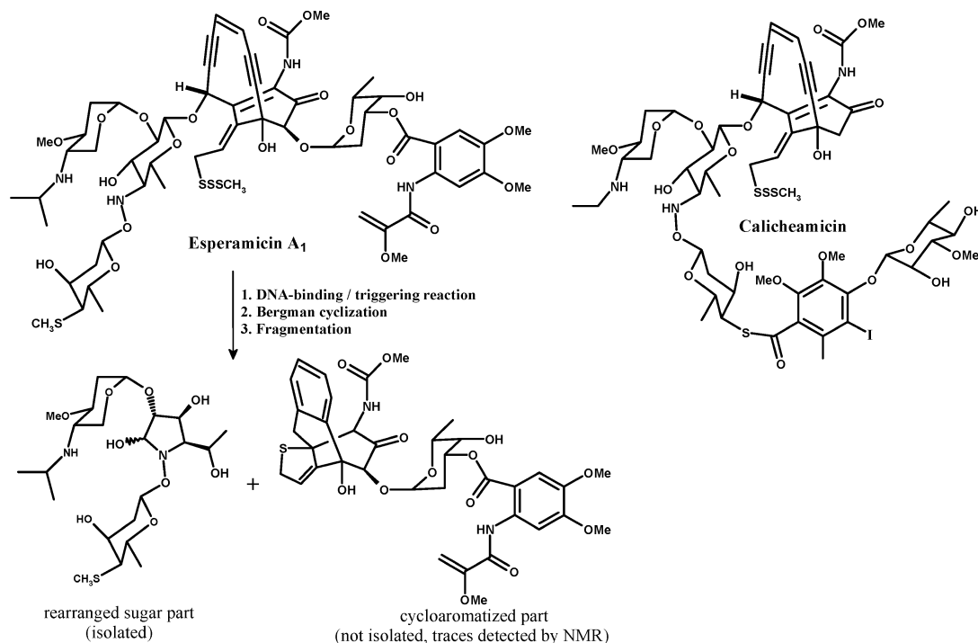
Figure 1. Structures of natural enediynes: esperamicin and calicheamicin.
