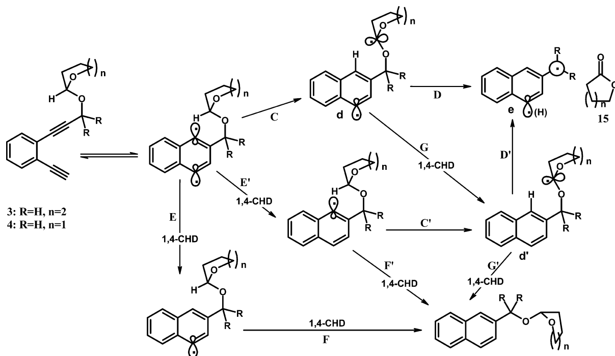
Scheme 11. Proposed Pathways for Bergman Cyclization/Fragmentation Cascades of Enediynes 3 and 4
