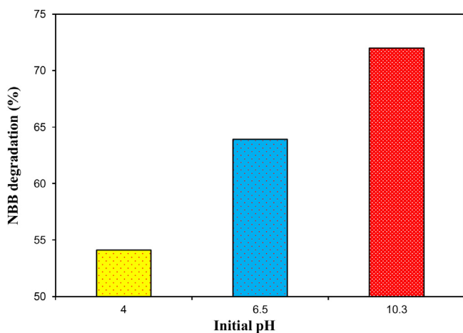
Fig. 6. Effect of solution pH; [NBB] = 30 ppm, dendrimer-ZnO suspension = 10 mg/50 mL, irradiation time = 60 min.
