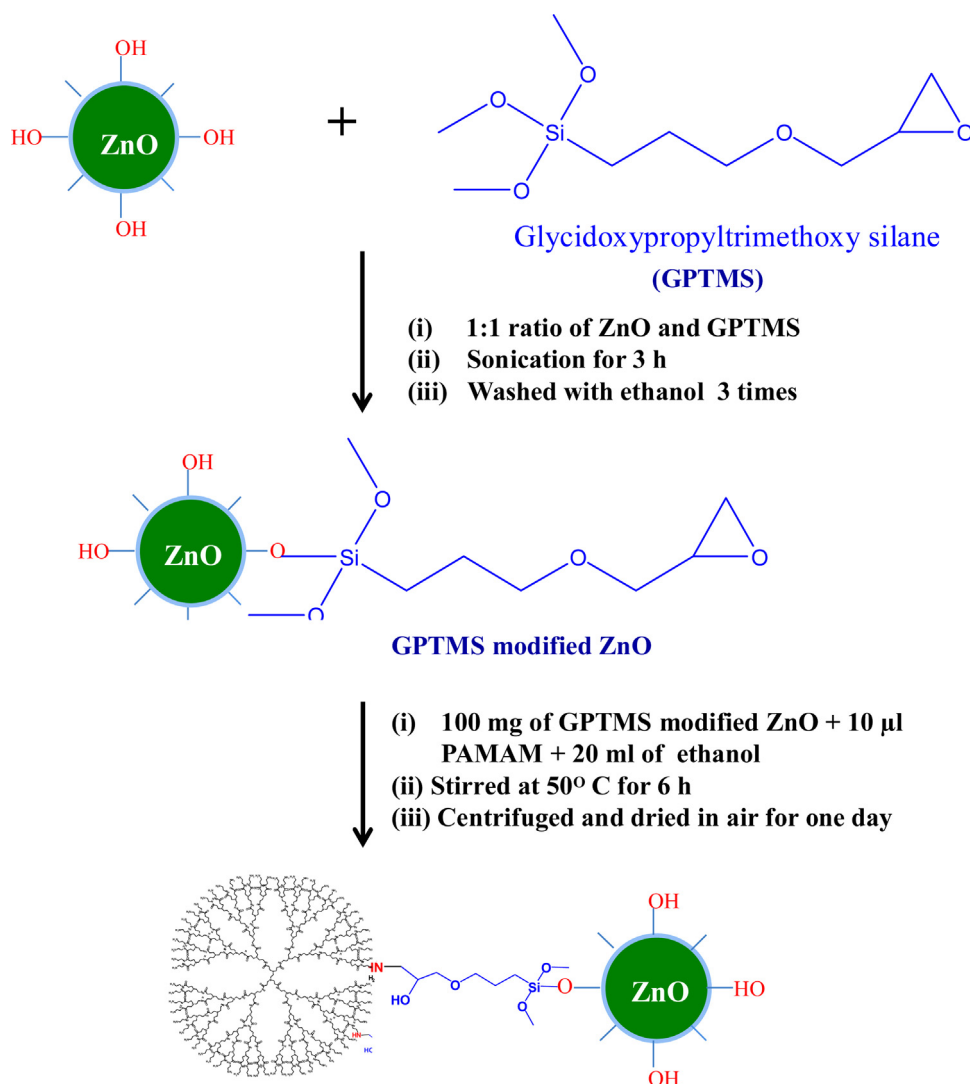
Scheme 1. Surface modification of ZnO by dendrimer using GPTMS.
