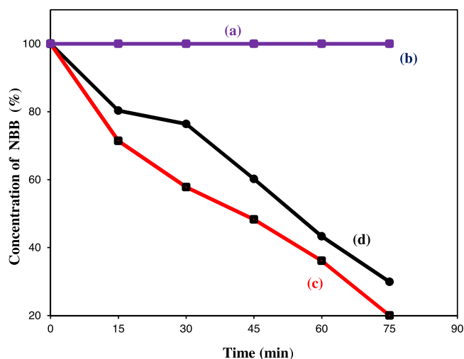
Fig. 5. Photodegradability of NBB; [NBB] = 30 ppm, catalyst suspension = 10 mg/50 mL, pH 6.5, (a) dendrimer-ZnO nanocomposite (dark, without irradiation), (b) no catalyst, (c) dendrimer-ZnO nanocomposite and (d) ZnO nano rods.
