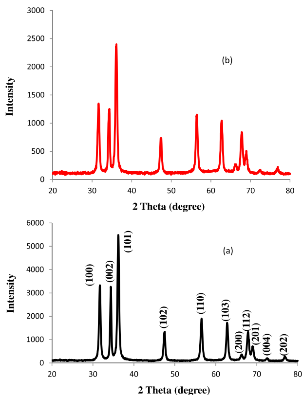
Fig. 1. XRD Patterns of (a) ZnO nano rods and (b) dendrimer-ZnO nanocomposite.
