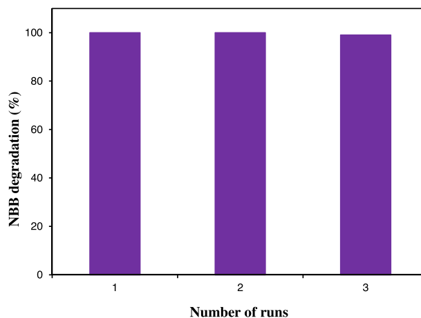
Fig. 8. Catalyst reusability; [NBB] = 30 ppm, dendrimer-ZnO suspension = 10 mg/50 mL, pH = 10.3, irradiation time = 90 min.
