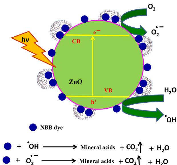
Scheme 2. Mechanism of degradation of NBB by dendrimer-ZnO nanocomposite.
