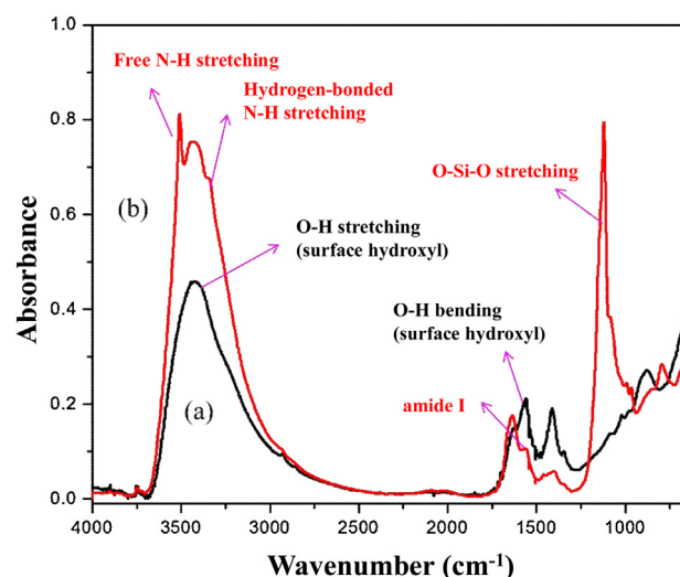
Fig. 2. IR spectra of (a) ZnO nano rods and (b) dendrimer-ZnO nanocomposite.
