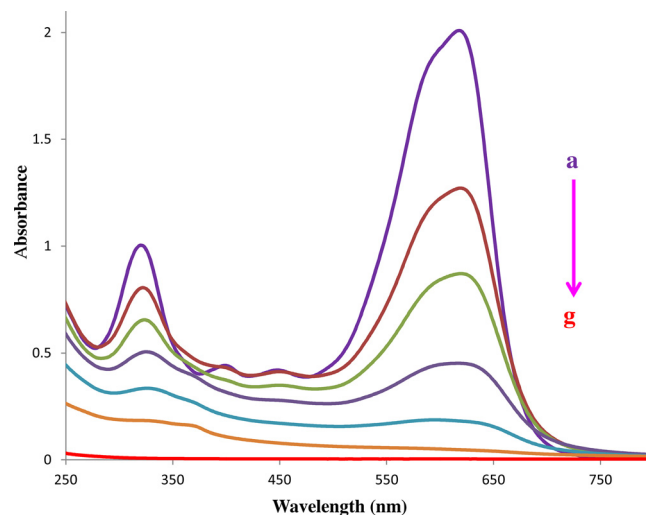
Fig. 7. UV-vis spectra of NBB after UV light irradiation in the presence of dendrimer-ZnO; [NBB] = 30 ppm, pH = 10.3, dendrimer-ZnO suspension = 10 mg/50 mL, irradiation time = (a) 0 min, (b) 15 min, (c) 30 min, (d) 45 min, (e) 60 min, (f) 75 min and (g) 90 min.
