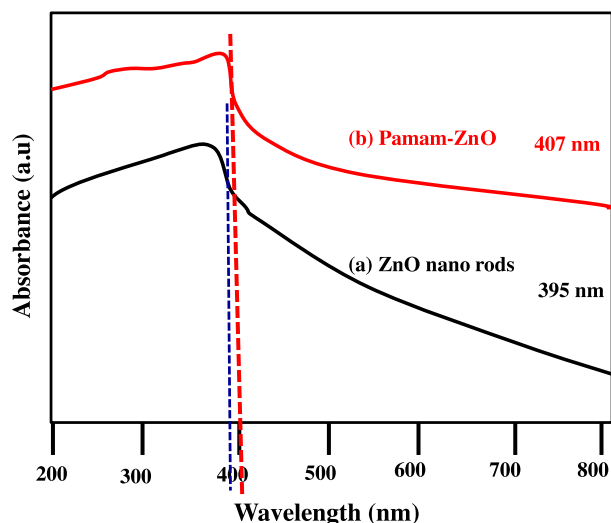
Fig. 4. DRS of (a) ZnO nano rods and (b) dendrimer-ZnO nanocomposite.
