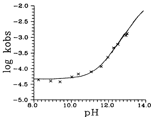
Figure 1. pH dependence of first-order rate constants for azobenzene formation in water-ethanol (97:3, v/v) at 25°C and ionic strength 1.0 M (KCl). The solid line was computed from equation (1) utilizing individual rate constants given in Table 1
