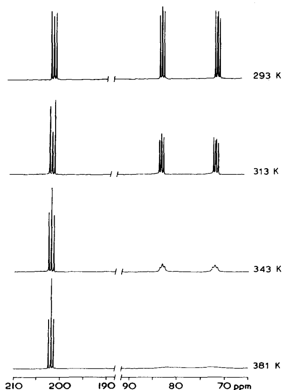
Fig. 1. Variable temperature ^{31}\text{P} NMR spectrum of 3 in toluene- d_8 .
