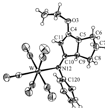
Figure 3. Molecular structure of the imine complex anti-11a . Selected bond lengths ( \text{\AA} ) and angles ( ^\circ ): \text{W}-\text{N12} = 2.276(3) , \text{N12}-\text{C10} = 1.296(5) , \text{N12}-\text{C120} = 1.452(5) , \text{C10}-\text{C9} = 1.528(5) , \text{C9}-\text{C8} = 1.547(6) , \text{C9}-\text{C5} = 1.559(5) , \text{C8}-\text{C7} = 1.526(6) , \text{C7}-\text{C6} = 1.528(6) , \text{C6}-\text{C5} = 1.520(6) , \text{C5}-\text{C4} = 1.503(5) , \text{C4}-\text{C11} = 1.348(5) , \text{C4}-\text{O3} = 1.327(5) , \text{C11}-\text{C10} = 1.434(5) ; \text{W}-\text{N12}-\text{C10} = 128.3(2) , \text{W}-\text{N12}-\text{C120} = 114.4(2) , \text{C120}-\text{N12}-\text{C10} = 117.1(3) , \text{N12}-\text{C10}-\text{C9} = 126.0(3) , \text{N12}-\text{C10}-\text{C11} = 125.0(3) , \text{C11}-\text{C10}-\text{C9} = 109.1(3) , \text{C10}-\text{C9}-\text{C8} = 113.2(3) , \text{C10}-\text{C9}-\text{C5} = 104.3(3) , \text{C5}-\text{C9}-\text{C8} = 104.2(3) , \text{C9}-\text{C8}-\text{C7} = 105.4(3) , \text{C8}-\text{C7}-\text{C6} = 102.4(4) , \text{C7}-\text{C6}-\text{C5} = 103.6(3) , \text{C6}-\text{C5}-\text{C4} = 112.8(3) , \text{C6}-\text{C5}-\text{C9} = 106.7(3) , \text{C9}-\text{C5}-\text{C4} = 102.7(3) , \text{C5}-\text{C4}-\text{O3} = 115.7(3) , \text{C5}-\text{C4}-\text{C11} = 114.1(3) , \text{O3}-\text{C4}-\text{C11} = 130.2(4) , \text{C4}-\text{C11}-\text{C10} = 109.4(3) .
