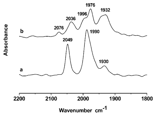
Figure 9. IR spectra in the CO region recorded during the electrolysis of 5 mM 2 with 50 mM HOAc in CO-saturated MeCN (0.1 M n -Bu 4 NPF 6 ) at -1.82 V: (a) prior to the application of the potential; (b) electrolysis for 2 h.
