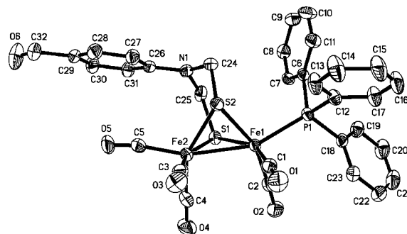
Figure 1. Molecular structure of 1 with 30% probability level ellipsoids.
