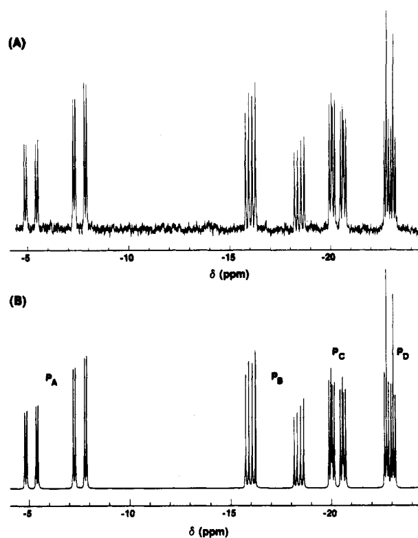
Figure 1. ^{31}\text{P}\{^1\text{H}\} NMR spectra for [\text{IrOs}(\text{CO})_3(\text{H})_2(\mu_2\text{-}\eta^3\text{-(}o\text{-C}_6\text{H}_4\text{)PhPCH}_2\text{PPh}_2\text{)}(\text{dppm})] (1): (A) observed (in d^8\text{-THF} ), (B) calculated.
