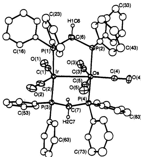
Figure 2. Perspective drawing of the [\text{IrOs}(\text{CO})_5(\text{dppm})_2]^+ cation showing the numbering scheme. The thermal ellipsoids are shown at the 20% level, except for the methylene hydrogens, which are drawn artificially small.
