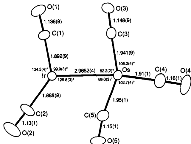
Figure 3. Representation of the metal-carbonyl plane showing some relevant parameters.
