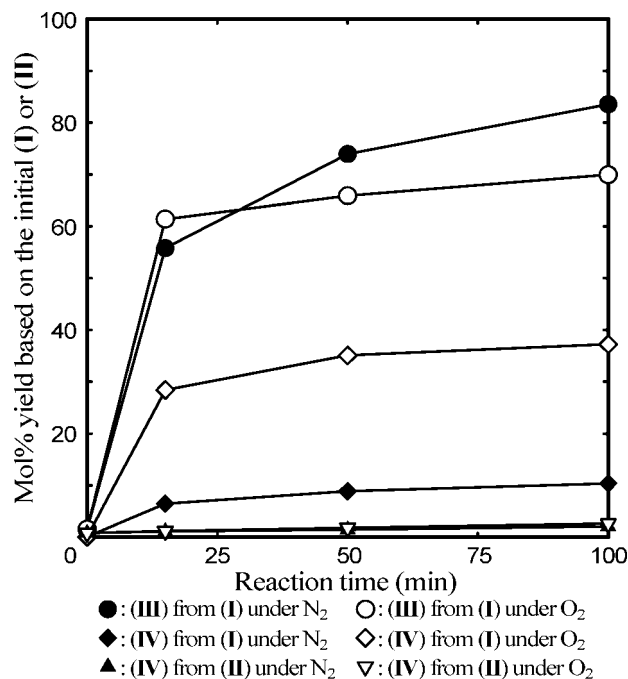
Figure 3. Yield of III and IV in the mild anaerobic alkaline and the oxygen-alkali treatments of I or II .
