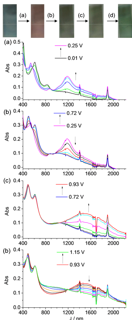
Figure 7. Absorption spectral changes of a poly- 2^+ /ITO film ( \Gamma = 1.0 \times 10^{-9} \text{ mol/cm}^2 ) upon stepwise applying potentials from (a) +0.01 to +0.25 V, (b) +0.25 to +0.72 V, (c) +0.72 to +0.93 V, and (d) +0.93 to +1.15 V vs Ag/AgCl. The plot on the top shows the film with different colors in different states.
