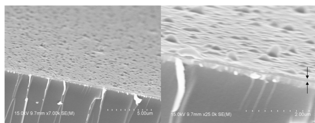
Figure 9. Representative SEM images of poly- 2^+ /ITO film ( \Gamma = 2.8 \times 10^{-9} \text{ mol/cm}^2 ). The polymeric layer (around 100 nm) is indicated by arrows.
