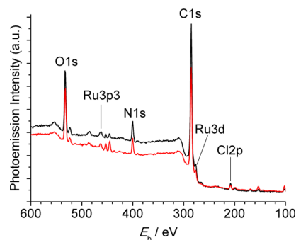
Figure 10. XPS survey spectra of poly- 1^+ /ITO (black curve) and poly- 2^+ /ITO (red curve) film.
