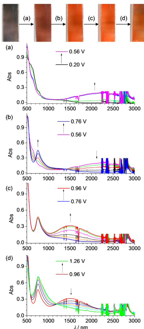
Figure 4. Absorption spectral changes of a poly-1 2+ film on ITO glass ( \Gamma = 4.2 \times 10^{-9} mol/cm 2 ) upon stepwise applying potentials from (a) +0.20 to +0.56 V, (b) +0.56 to +0.76 V, (c) +0.76 to +0.96 V, and (d) +0.96 to +1.26 V vs Ag/AgCl. The plot on the top shows the film with different colors in different states.
