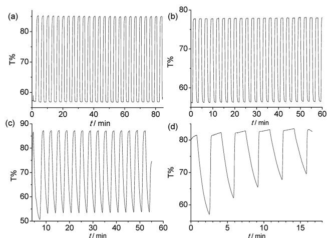
Figure 8. Transmittance switching of a poly- 2^+ /ITO film ( \Gamma = 5.5 \times 10^{-9} \text{ mol/cm}^2 ) monitored at \lambda = (a,b) 1185 nm and (c,d) 1600 nm as a function of time ( t ) between (a) +0.01 and +0.43 V, (b) +0.43 and +0.70 V, (c) +0.70 and +0.93 V, and (d) +0.93 and +1.20 V vs Ag/AgCl in 0.1 M \text{Bu}_4\text{NClO}_4/\text{CH}_2\text{Cl}_2 .
