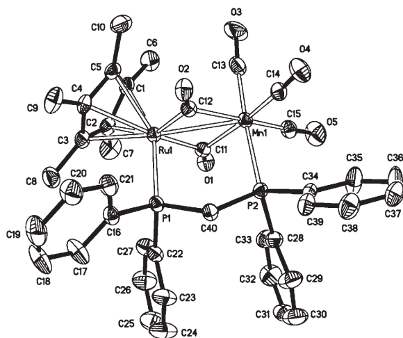
Figure 2. X-ray structure of [\text{C}_5(\text{CH}_3)_5]\text{Ru}(\mu\text{-CO})_2(\mu\text{-dppm})\text{Mn}(\text{CO})_3 ( 1b ).
