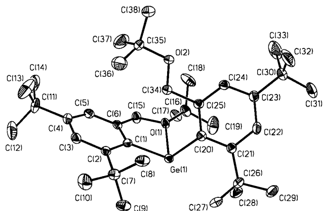
Figure 2. Molecular structure of 2 (50% probability).
