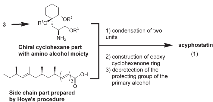
Scheme 2. Summary of the synthesis of scyphostatin ( 1 ).
