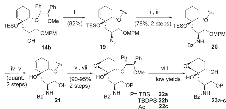
Scheme 6. Introduction of a nitrogen atom into 14b . i) DPPA, PPh 3 , DEAD, THF, RT; ii) LiAlH 4 , THF, 0°C; iii) BzCl, Et 3 N, CH 2 Cl 2 , RT; iv) DDQ, CH 2 Cl 2 , RT; v) TBAF, THF, RT; vi) TBSCl, imidazole, DMF, RT for 22a ; TBDPSCl, imidazole, DMF, RT for 22b ; Ac 2 O, pyridine, RT for 22c ; vii) TBHP, [VO(acac) 2 ], toluene, RT; viii) 1. [Pd(OH) 2 ], H 2 , MeOH, RT, 3.5 atm or 2. liq. NH 3 , ca. −78°C. acac = acetylacetonate, DDQ = 2,3-dichloro-5,6-dicyano-1,4-benzoquinone, TBAF = tetra- n -butylammonium fluoride, TBDPSCl = tert -butyldiphenylsilyl chloride, TBSCl = tert -butyldimethylsilyl chloride.
