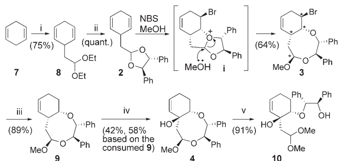
Scheme 3. Synthesis of cyclohexene dimethyl acetal 10 . i) sec -BuLi, TMEDA, THF, -78°C, then BrCH 2 CH(OEt) 2 ; ii) ( R,R )-hydrobenzoin, p -TsOH, toluene, 50°C; iii) Bu 3 SnH, AIBN, benzene, reflux; iv) SeO 2 , pyridine, dioxane, 70°C; v) cat. PPTS, MeOH, RT. AIBN = azobisisobutyronitrile, PPTS = pyridinium p -toluene sulfonate, TMEDA = N,N,N',N' -tetramethylethylenediamine, p -TsOH = p -toluenesulfonic acid.
