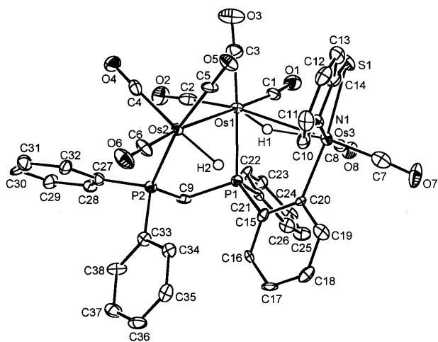
Fig. 2. Molecular structure of [\text{H}(\mu\text{-H})\text{Os}_3(\text{CO})_8(\eta^2\text{-pyS})\{\text{Ph}_2\text{PCH}_2\text{P(Ph)C}_6\text{H}_4\}] ( 5 ) showing the atom labeling. Thermal ellipsoids are drawn at 50% probability level. The hydrogen atoms except those bonded to the osmium atoms are omitted for clarity.
