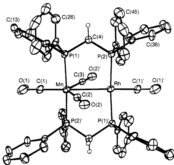
Figure 1. Perspective view of [\text{RhMn}(\text{CO})_4(\text{dppm})_2] (5) showing the numbering scheme. Thermal parameters are shown at the 20% level except for hydrogens, which are shown artificially small for the methylene groups but are not shown for the phenyl groups. Although the molecule is inversion-disordered, only one of the two positions for each of C(2) and C(3) is shown and the two disordered Rh/Mn positions are identified as assumed for the ordered structure.
