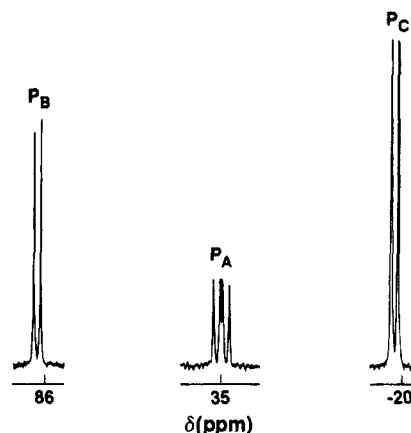
Figure 3. ^{31}P\{^1H\} NMR spectrum at 22 °C for [RhFeCp(CO)(dppm)_2] ( 9 ).
