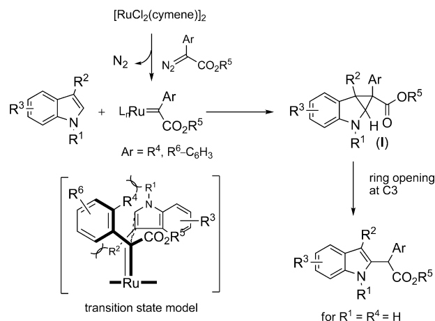
Scheme 1. Proposed Mechanism and Transition State Model
