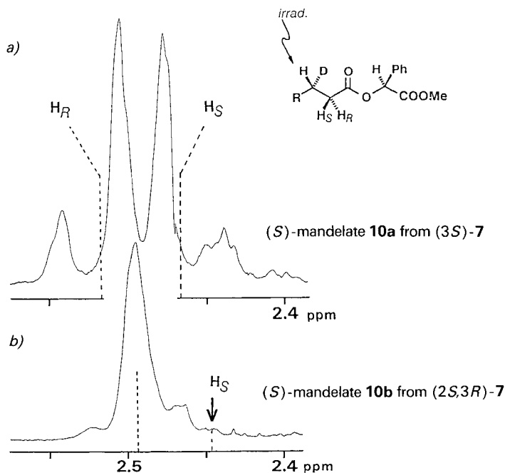
Fig. 1. 400-MHz ^1\text{H-NMR} spectra ( \text{CDCl}_3 ) of mandelate diesters: a) mandelate diester 10a prepared from (3 S )-7; b) mandelate diester 10b prepared from (2 S ,3 R )-7. Spectra are recorded with irradiation at 2.35 ppm of the adjacent methylene group (H–C(3)). The highfield shift of 0.026 ppm for the anisochronous H–C( \alpha ) of 10b as compared to 10a is due to the presence of the additional ^2\text{H} -atom at C(2) in 10b .
