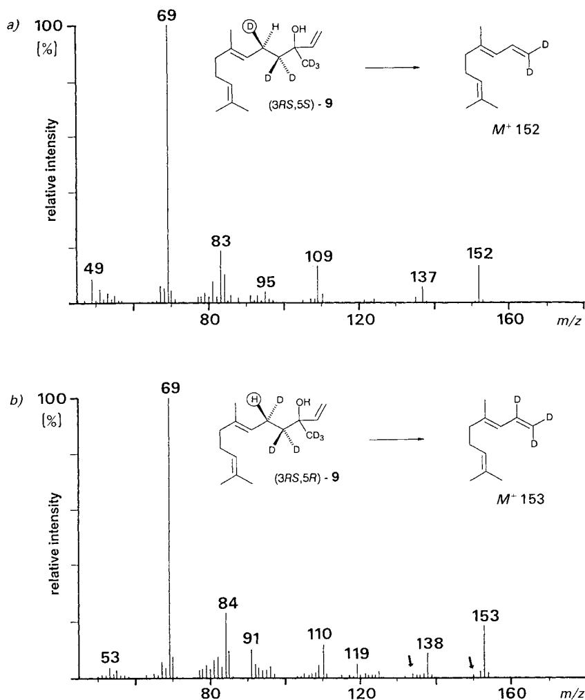
Fig. 3. EI-MS (70 eV) Analysis of artificial metabolites from Yucca filamentosa . Spectra are taken out of the front area of the eluting homoterpenes. a) MS of (1,1,2- H_2 )-1 from incubation with (3RS,5S)-9; b) MS of (1,1,2- H_3 )-1 from incubation with (3RS,5R)-9. Arrows indicate the small contamination by natural ( ^1H )-1. The H_5 -C(5) is enantiospecifically removed upon the oxidative bond cleavage. Conditions: Finnigan MAT 90 GC/MS. Separation of the compounds was achieved on a BP 5 fused silica column (25 m \times 0.32 mm) under programmed conditions (70° for 5 min, then at 12°/min to 250°). Scan range: 45–300 Da/s.
